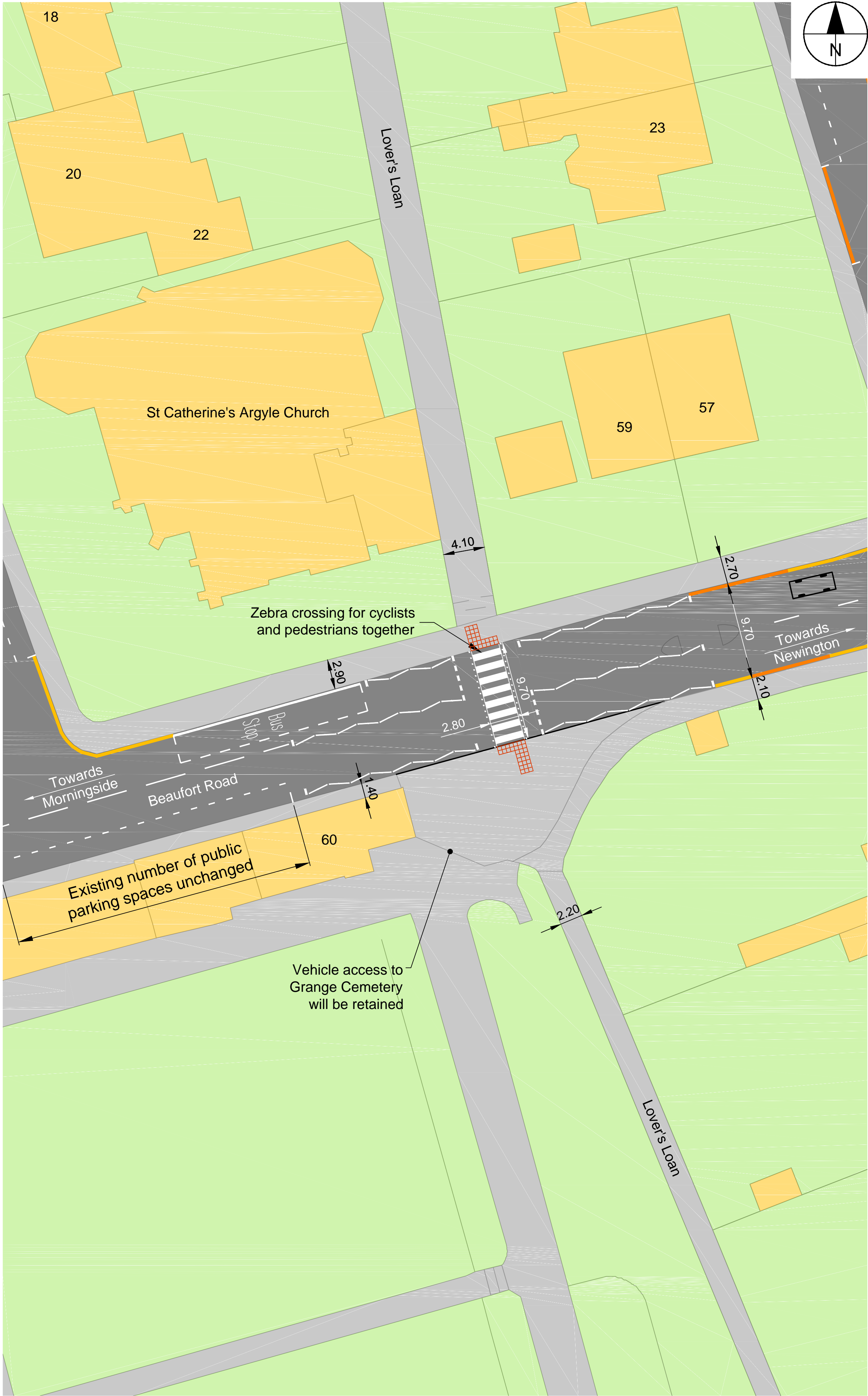
Proposed Layout
