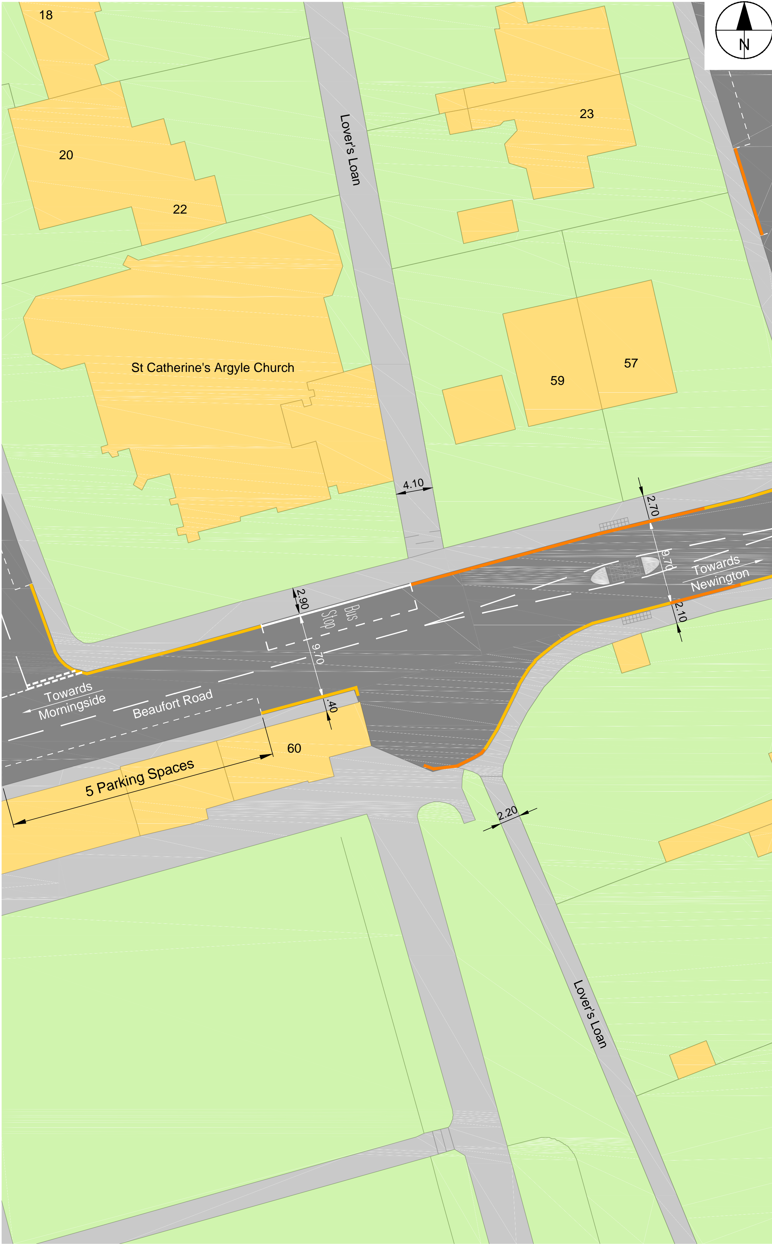
Existing Layout
