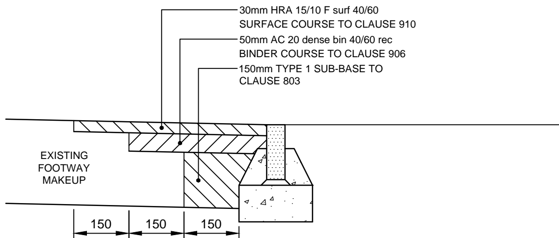
REINSTATEMENT OF FOOTWAY
