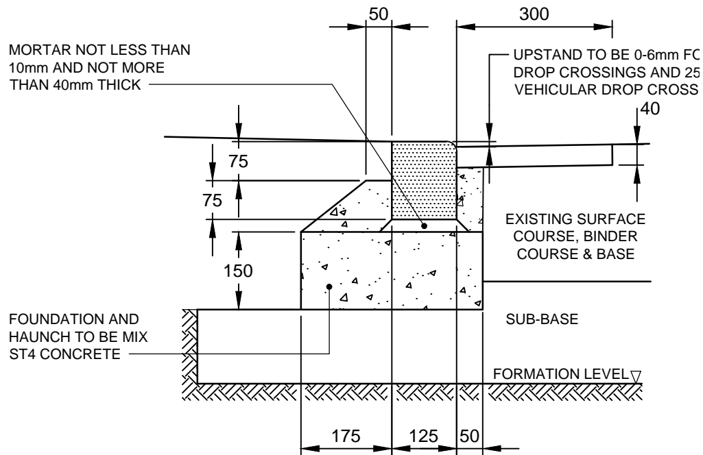
PRECAST CONCRETE ROAD KERB 125 x 150mm BULLNOSE PATTERN
