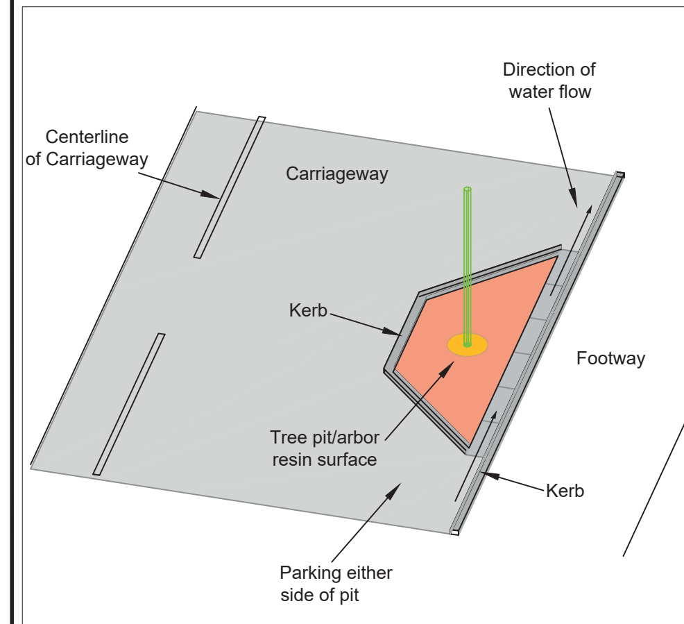
Typical Tree Pit Detail A
