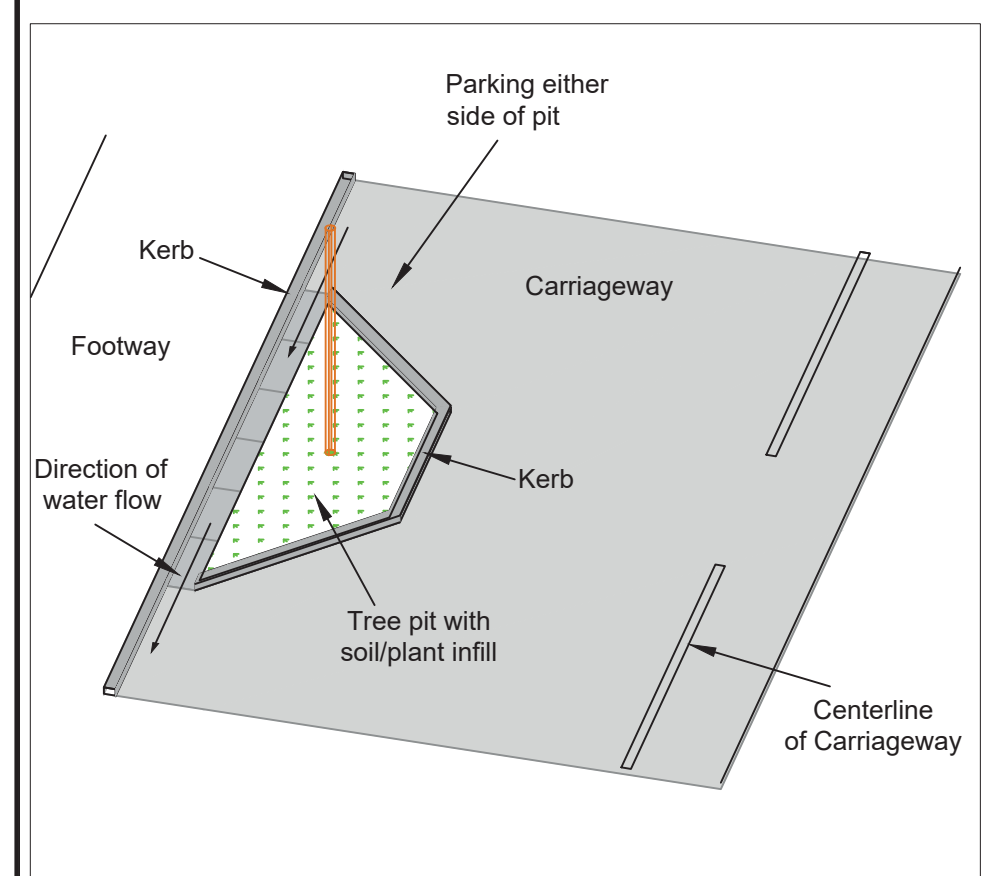
Typical Tree Pit Detail B
